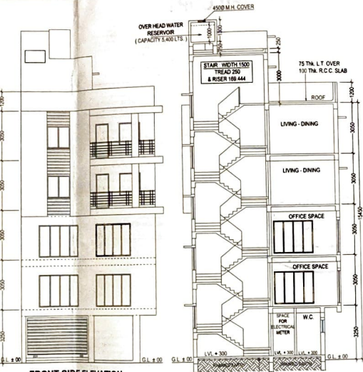
SECTION THROUGH, X - X'.
