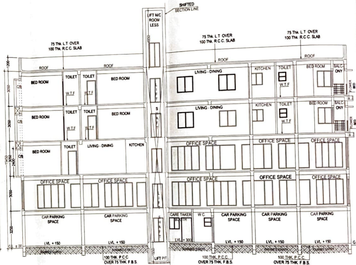
SECTION THROUGH, Y - Y'.
