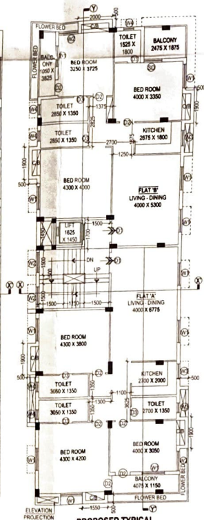
PROPOSED TYPICAL (3RD & 4TH) FLOOR PLAN
